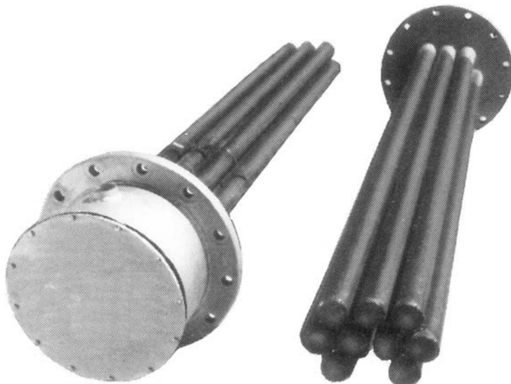
Flanged Immersion Heater using withdrawable elements
