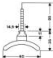
Element complete with mounting clips
