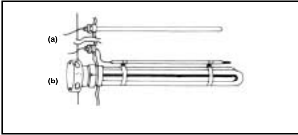
Fig. 8 Thermostat bulb installed in a tank: a) in a well; b) adjacent to an immersion heater.
