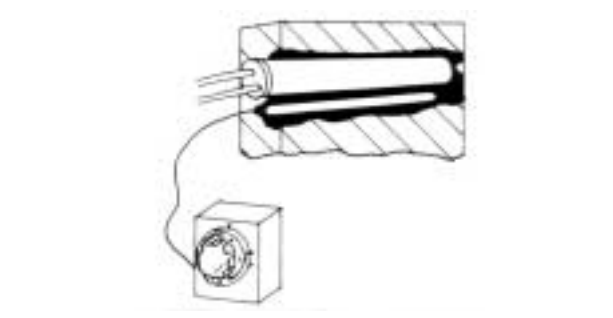
Fig.11 Cartridge heater and thermostat bulb inserted into machined holes.
